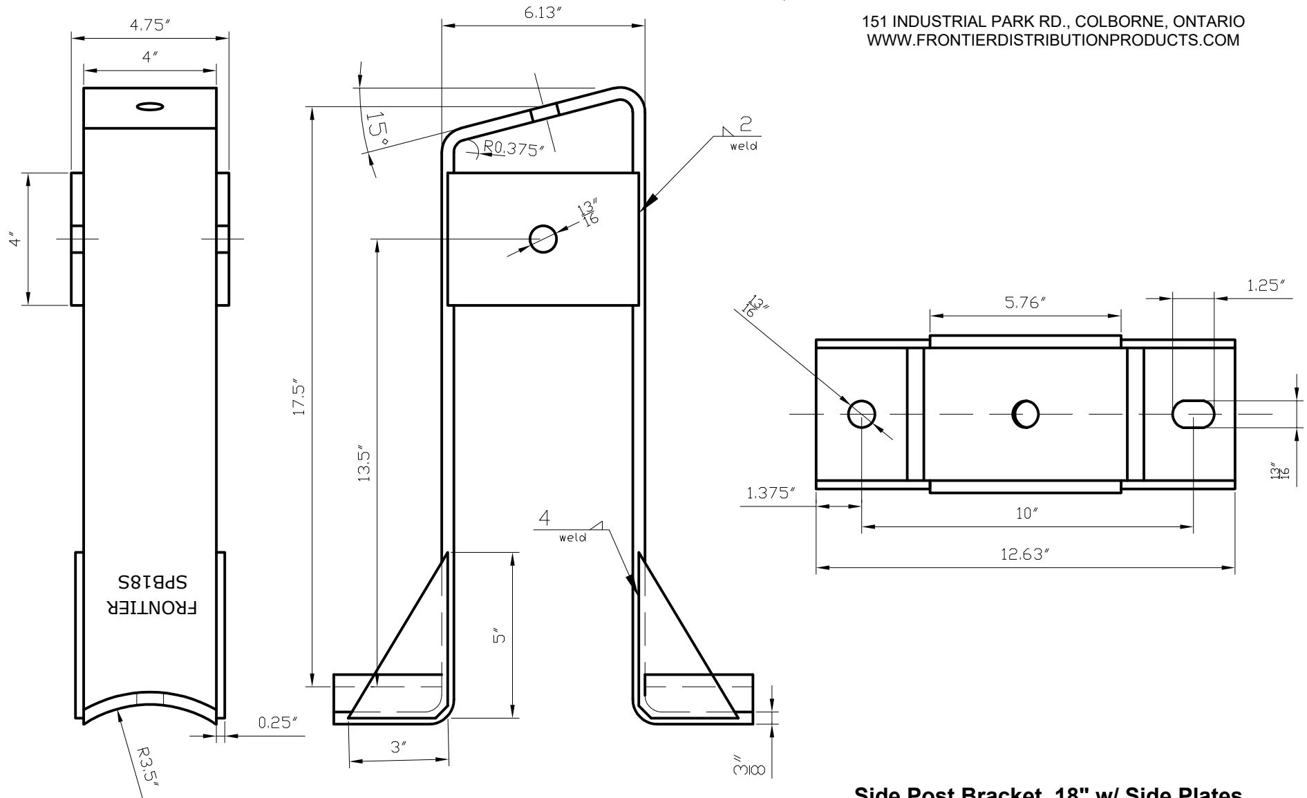
Side Post Bracket, 18" w/ Side Plates
