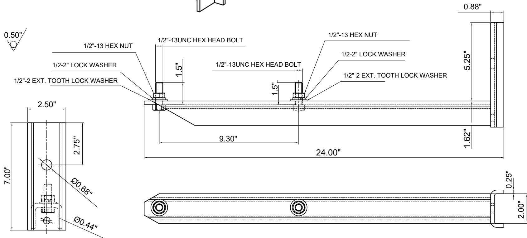
Cut Out / Arrester Bracket
